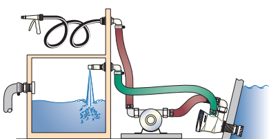
High Pressure Washdown plus Livewell
