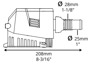
Sahara Mk2 1200 with Outlet - Straight
