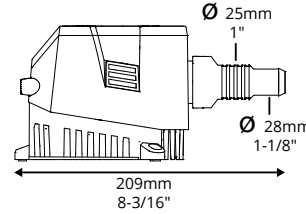
Sahara Mk2 500/800 with Outlet - Straight
