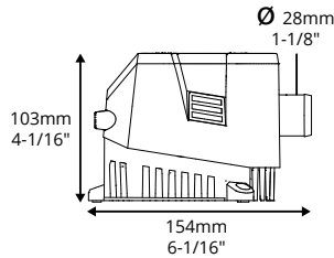
Sahara Mk2 1200 Barb
