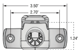
Vertical Composite Base
